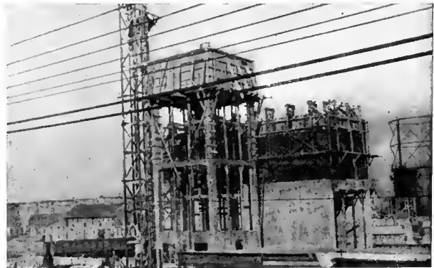
COKE QUENCHING PLANT DURING CONSTRUCTION
